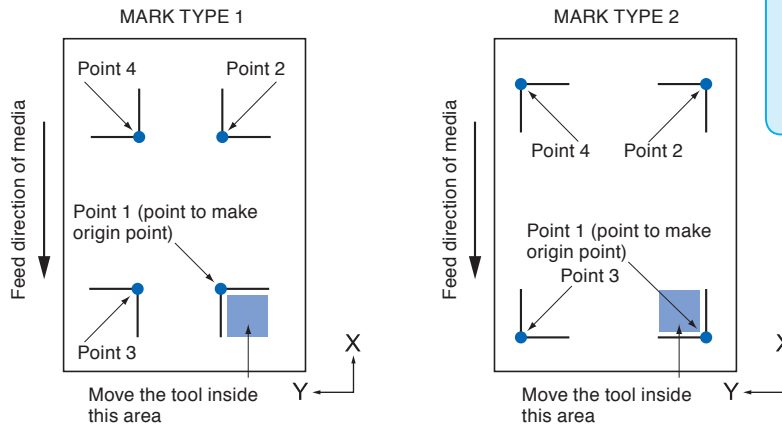
Registration mark scan start area
